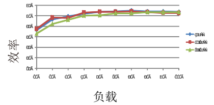
DDR-120C-48
