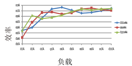
DDR-120D-48
